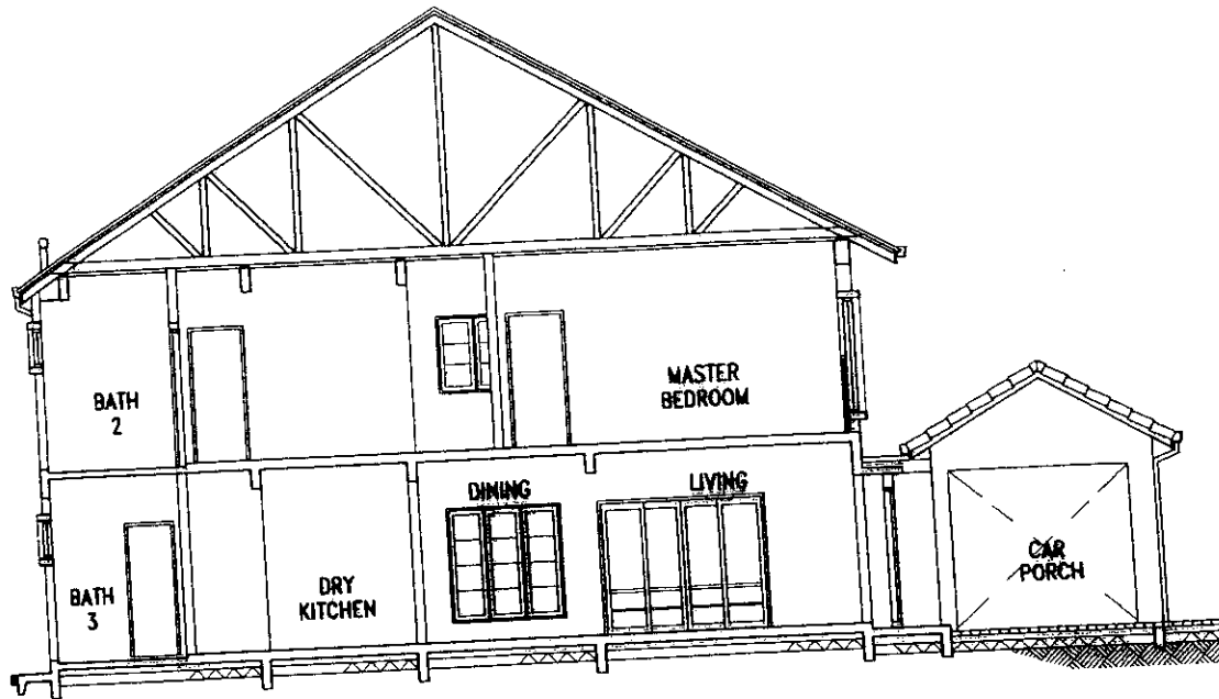
SECTIONAL ELEVATION TYPE B1
