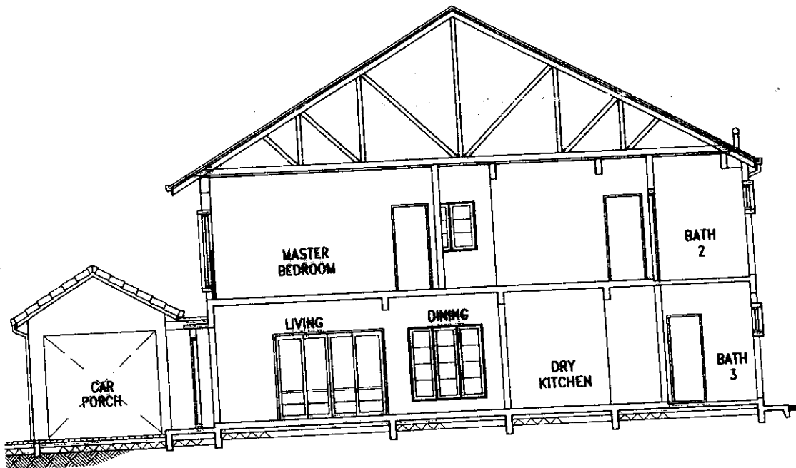
SECTIONAL ELEVATION TYPE B1
